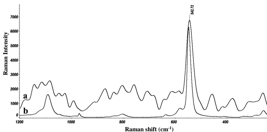
Figure 2: (a): \mu -Raman spectrum (excitation laser wavelength: 532 nm) of blue pigment with code "d" compared to (b): ultramarine spectrum (RRUFF ID: R040023) and observation of its index peak at 543 \text{ cm}^{-1} .
