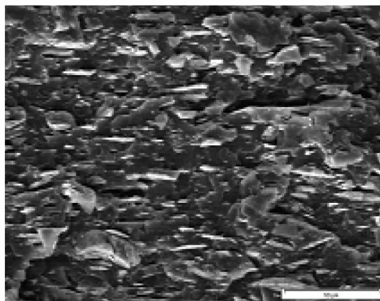
(ج) PP+20%Talc+10%Resin(600X)
